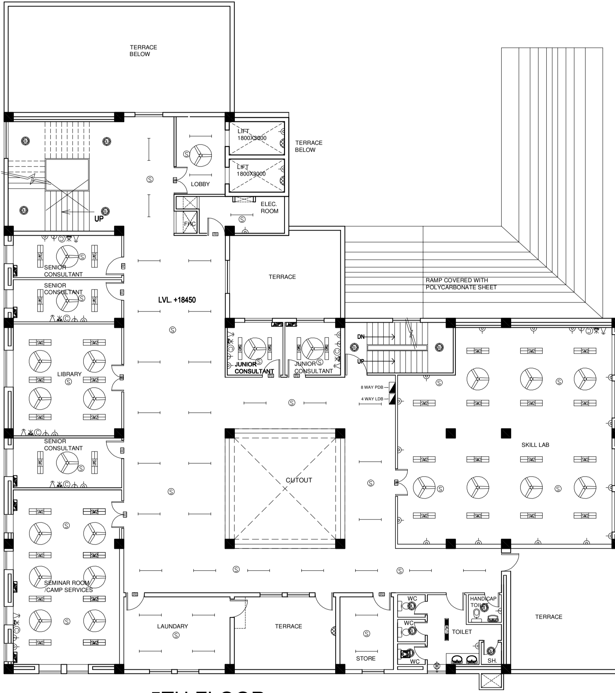
5TH FLOOR
