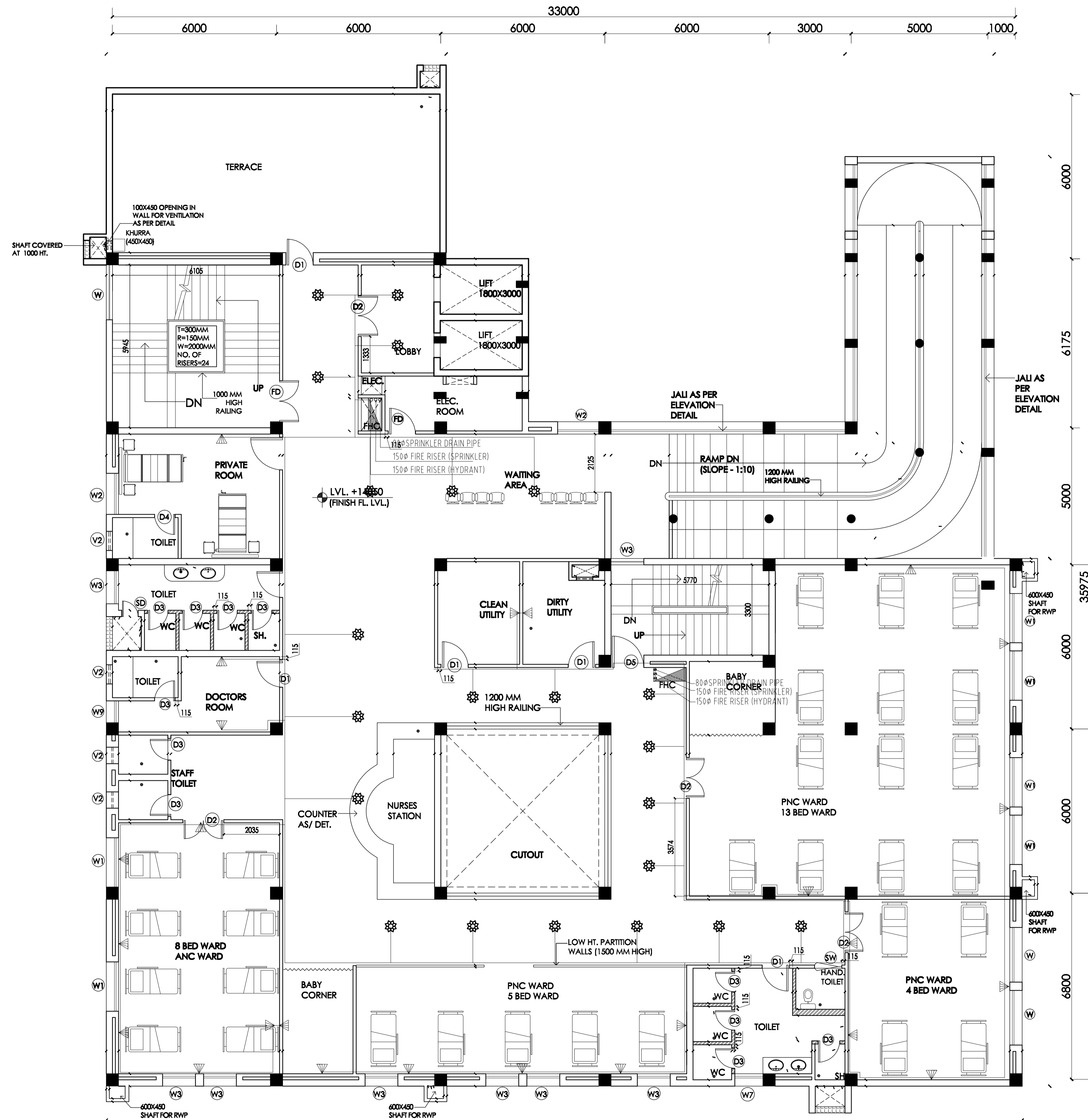
4TH FLOOR - POST NATAL CARE WARD - 30 BEDS
