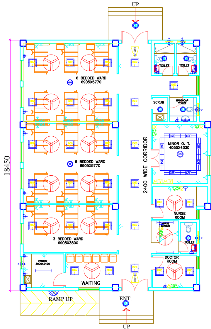
GROUND FLOOR AREA - 250 SQM
