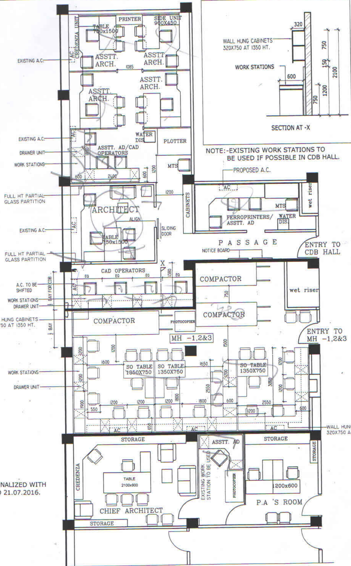
LAYOUT OF CDB HALL
