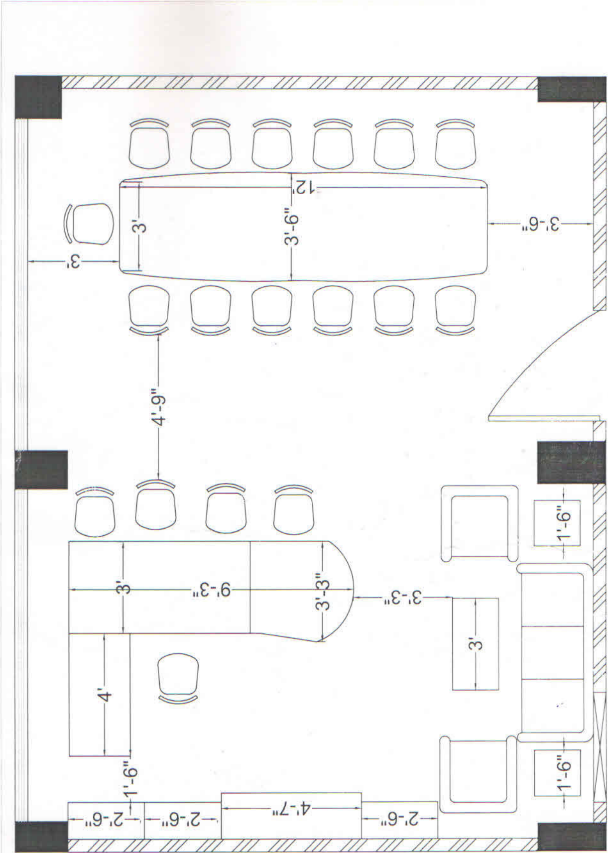
ROOM NO. - 158 - A
