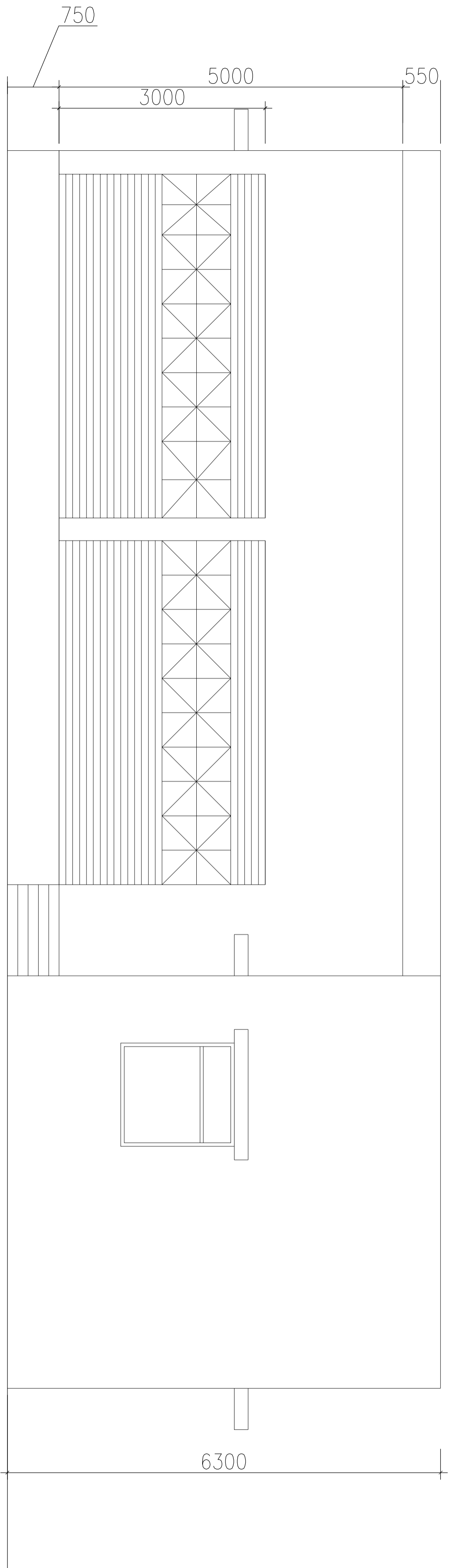
FRONT ELEVATION
